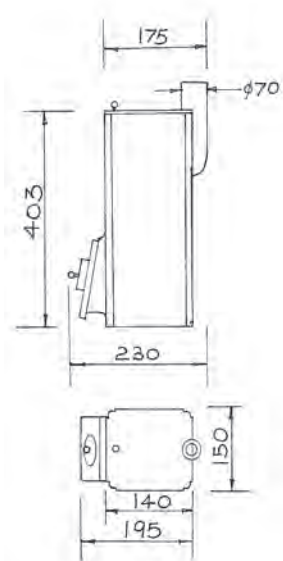
3126/BR Stove with brass fitments
